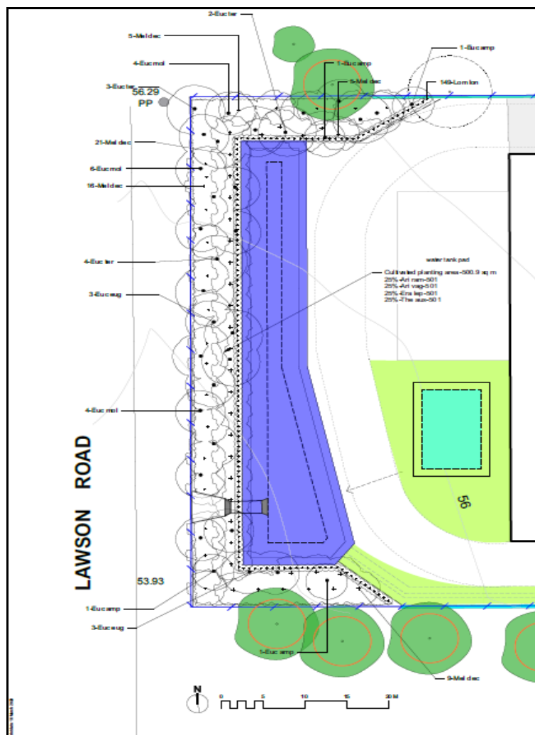
PLANTING PLAN - LAWSON ROAD FRONTAGE
